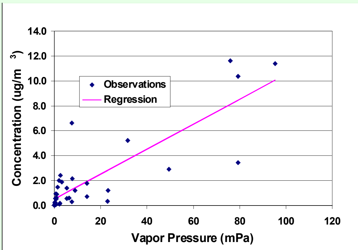
Figure 2. Relationship between maximum pesticide comparison in air above turf and chemical vapor pressure.
